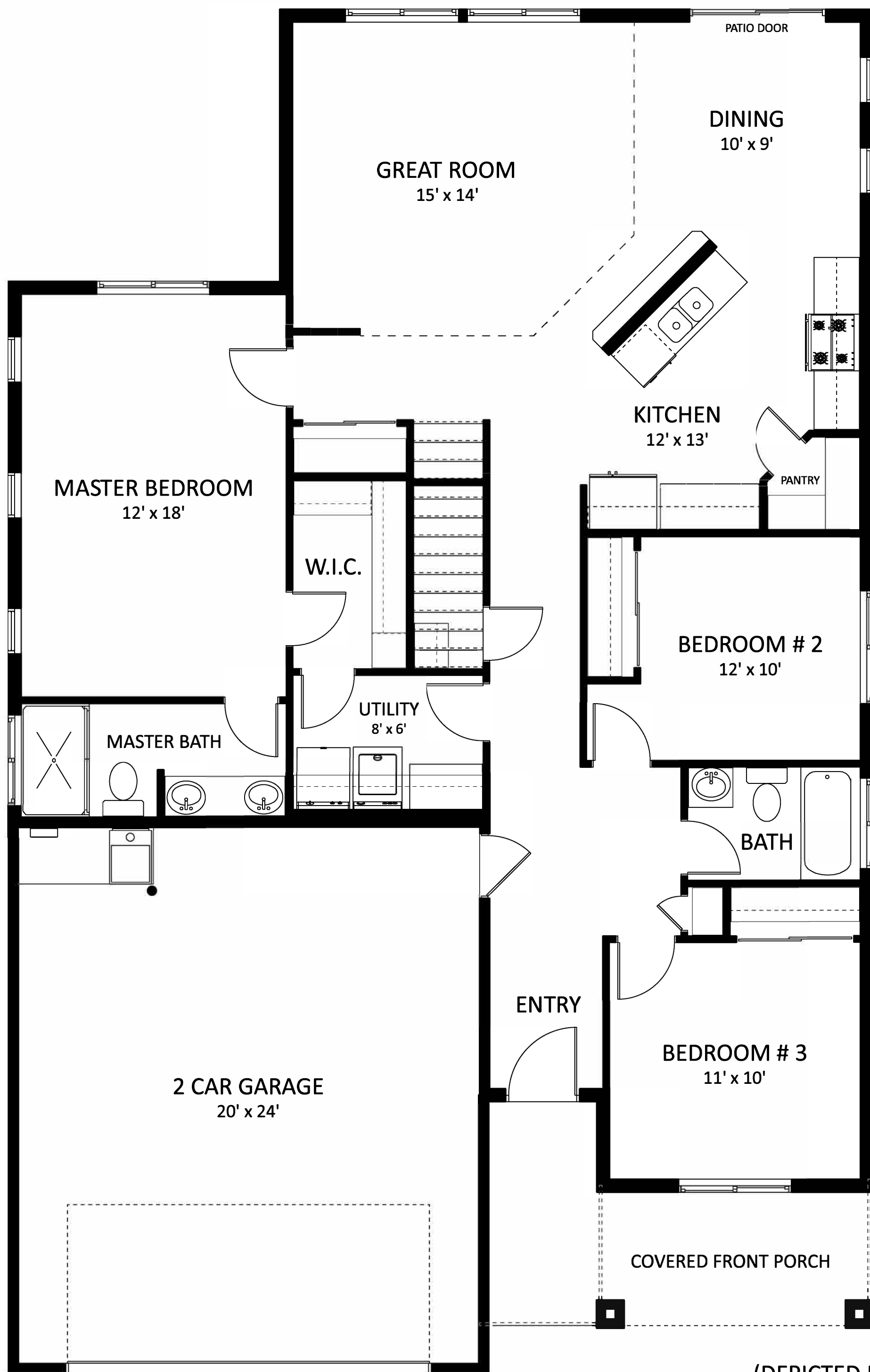
MAIN FLOOR
